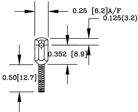
SCREW 6 BA Brass, Nickel Plated
