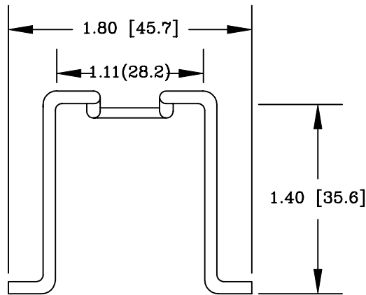
CLIP .072" Dia. Stainless Steel Wire
